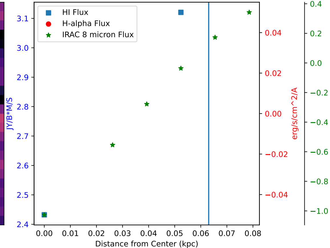
Flux of HI vs. H-alpha in Galaxy: DDO 53 - Region 3
